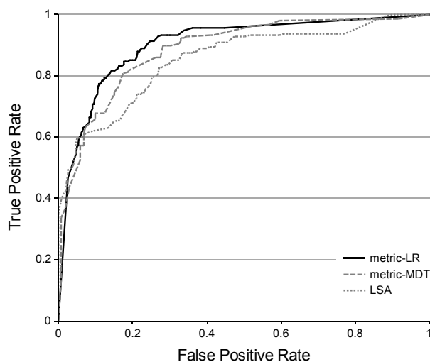
Figure 1. ROC for different similarity measures on the grouping task: trained metrics using logistic regression and a mixture of decision trees (MDT) as well as LSA.
