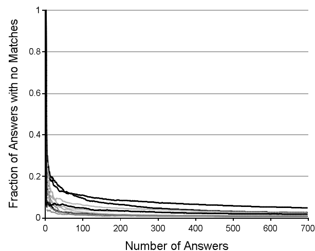
Figure 9. Fraction of answers with no match from another student using the learned similarity metric; each curve represents one question, and the x-axis represents the size of the answer set (i.e., class size). Each curve is averaged over 30 reshufflings of the answer set.
